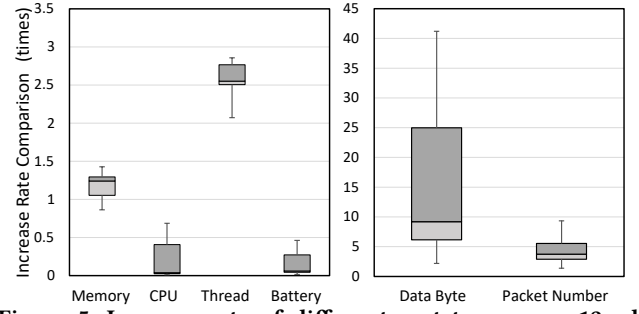
Figure 5: Increase rate of different cost types over 12 ad schemes.
