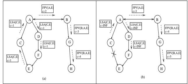
Figure 2: Basic HLP route propagation: Link failure example
