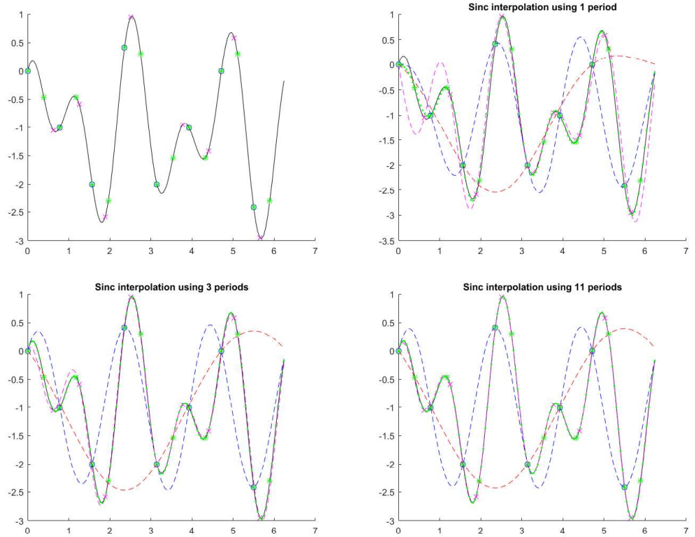
Figure 1: Top Left : The function \cos(5t) + \sin 3t - 1 sampled at different rates : + 4 samples in period, \circ 8 samples per period, \times 10 samples per period (i.e. the Nyquist rate), * 16 samples per period. Top Right : Reconstruction of the function at 128 sampling points from Eq. 23 using n = 1 ; - reconstruction from 4 samples in period, - reconstruction from 8 samples per period, - reconstruction from 10 samples per period (i.e. the Nyquist rate), - reconstruction from 16 samples per period. Bottom Left : As Top Right with n = 3 . Bottom Right : As Top Right with n = 11 .
